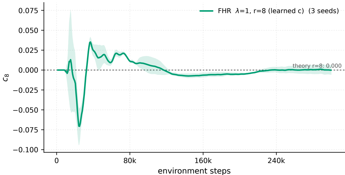
MountainCarContinuous-v0 - recurrence coefficient c_8 vs the Bellman theory value
