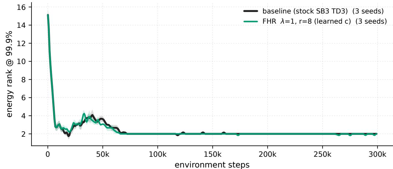
MountainCarContinuous-v0 - \lambda 1 \cdot r8 vs baseline, penalised windows energy rank @ 99.9%
