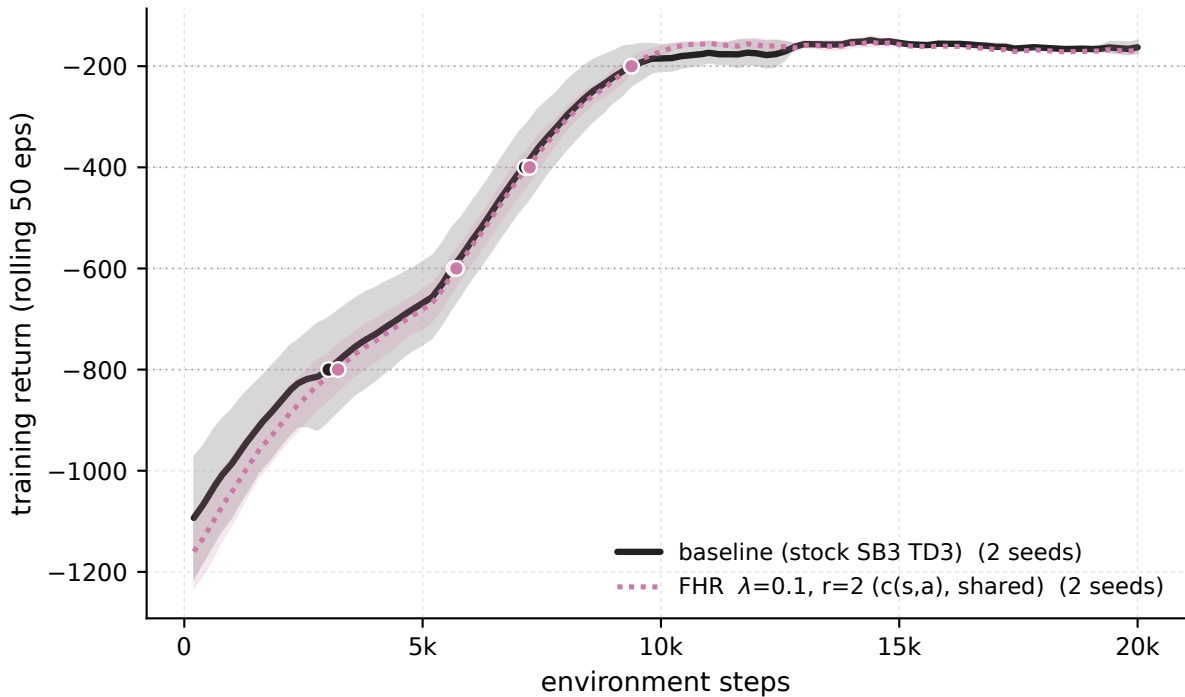
Pendulum-v1 - \lambda 0.1 \cdot r_2 c(s,a) shared vs baseline (training stream)
