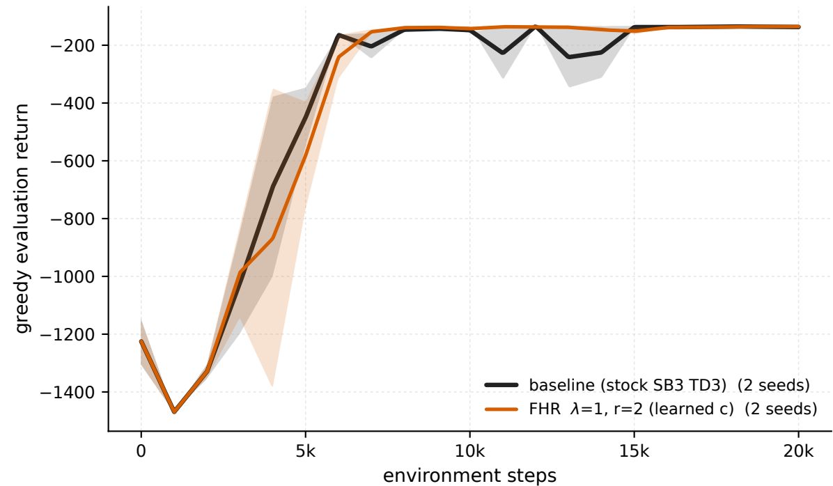
Pendulum-v1 - \lambda 1 \cdot r_2 vs baseline (greedy eval)
