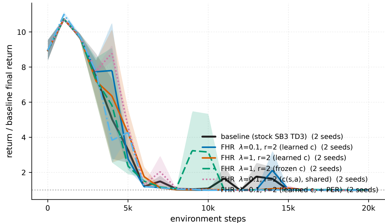
Pendulum-v1 - all arms, baseline-normalised (eval)
