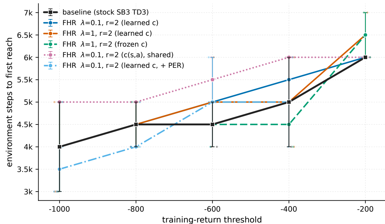
Pendulum-v1 - sample efficiency, greedy-eval stream (mean \pm 1 s.e.m.)
