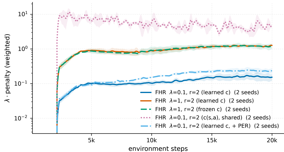
Pendulum-v1 - \lambda \cdot \text{penalty} (weighted)
