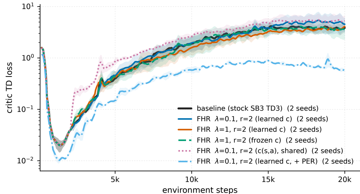
Pendulum-v1 - critic TD loss
