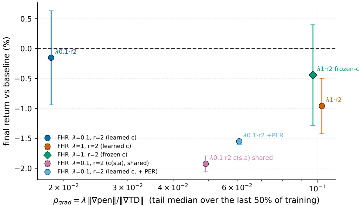
Pendulum-v1 - how hard the penalty pushes vs what it buys
