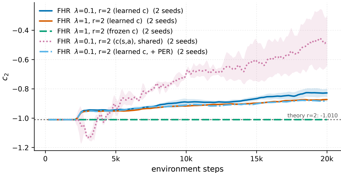
Pendulum-v1 - recurrence coefficient c_2 vs the Bellman theory value
