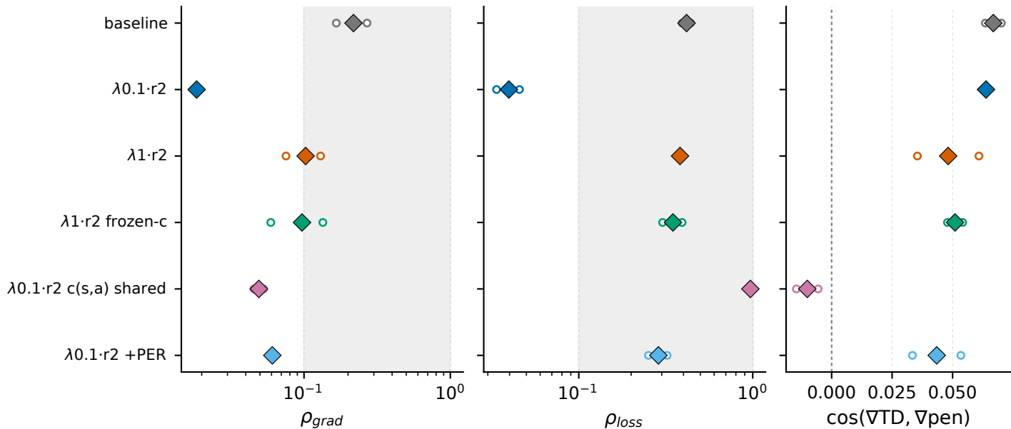
Pendulum-v1 - stream ratios, tail medians over the last 50% (baseline: unweighted); shaded = target range
