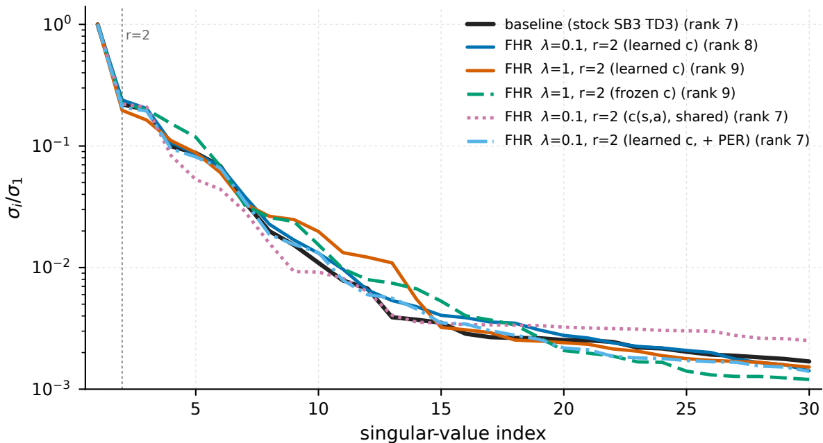
Pendulum-v1 - Hankel( Q(s_t, \pi(s_t)) ) of the final policy (critic trace)
