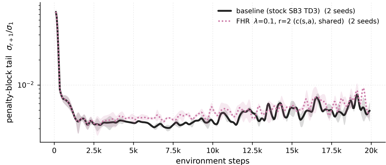
Pendulum-v1 - \lambda 0.1 \cdot r_2 c(s,a) shared vs baseline, penalised windows penalty-block tail \sigma_{r+1}/\sigma_1
