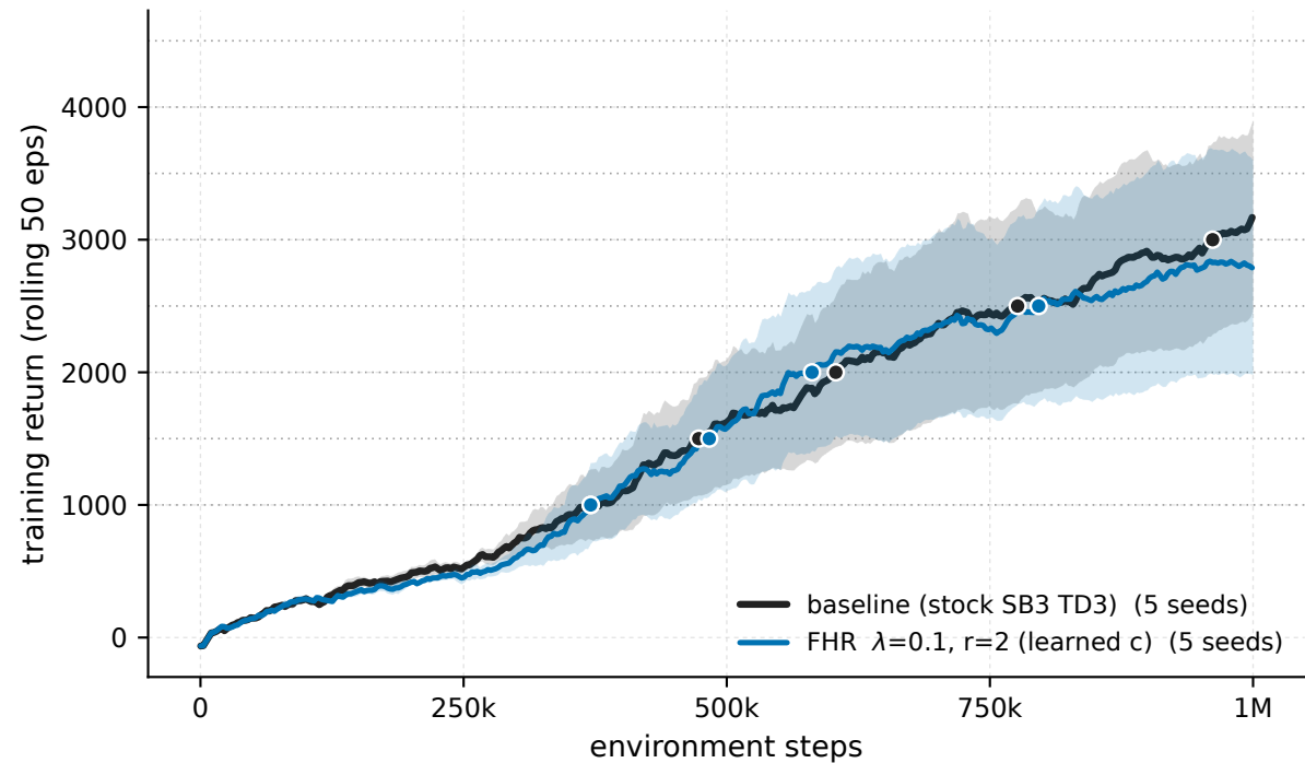
Ant-v5 - \lambda 0.1 \cdot r_2 vs baseline (training stream)
