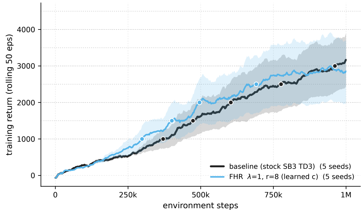
Ant-v5 - \lambda 1 \cdot r 8 vs baseline (training stream)
