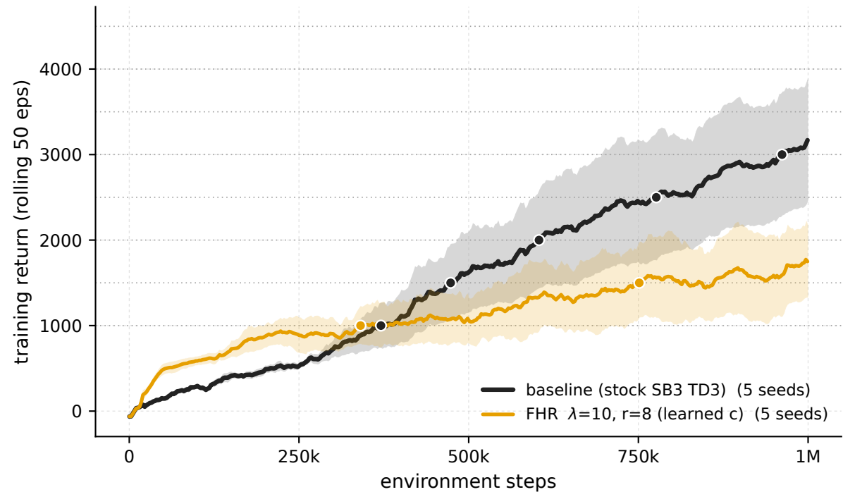
Ant-v5 - \lambda 10 \cdot r8 vs baseline (training stream)
