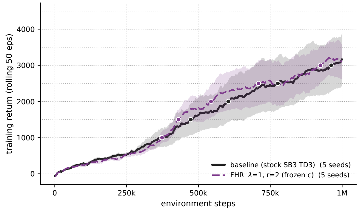
Ant-v5 - \lambda 1 \cdot r2 frozen-c vs baseline (training stream)
