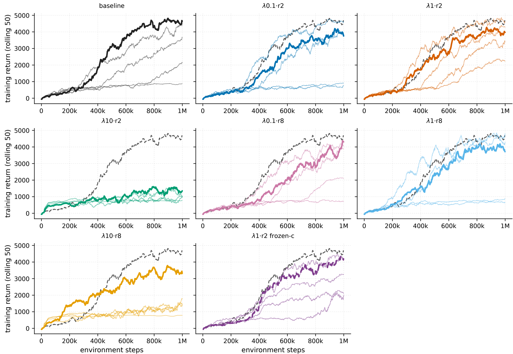
Ant-v5 - every seed per arm (train); grey dashed = baseline seed mean
