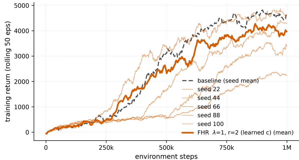
Ant-v5 - \lambda 1 \cdot r2 , every seed (train)
