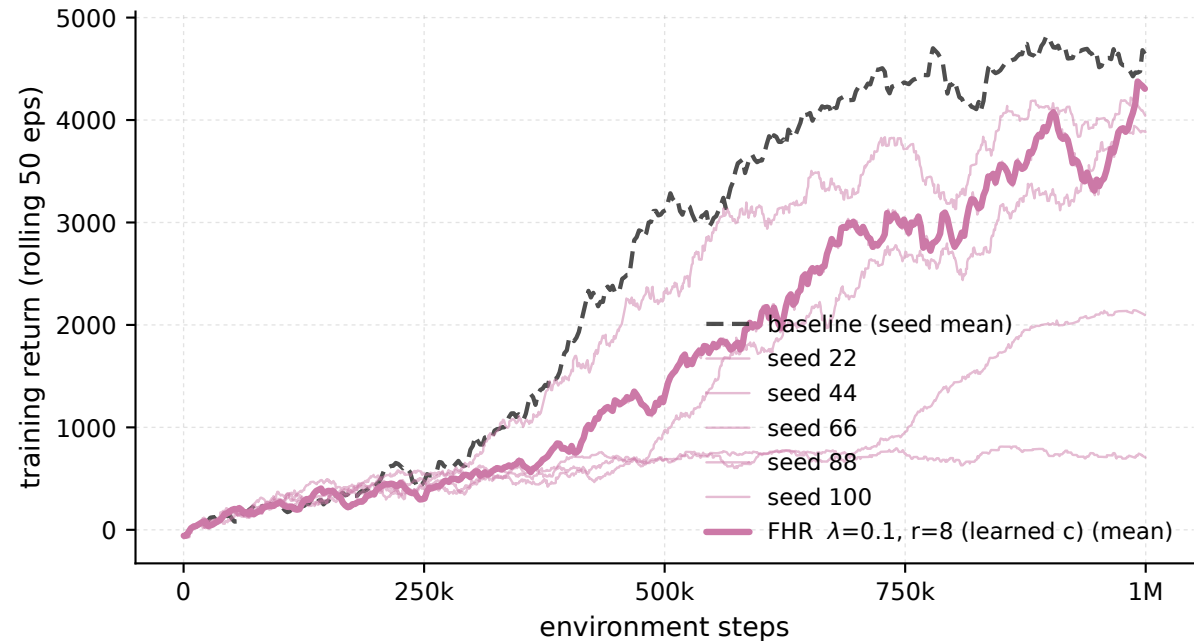
Ant-v5 - \lambda 0.1 \cdot r8 , every seed (train)
