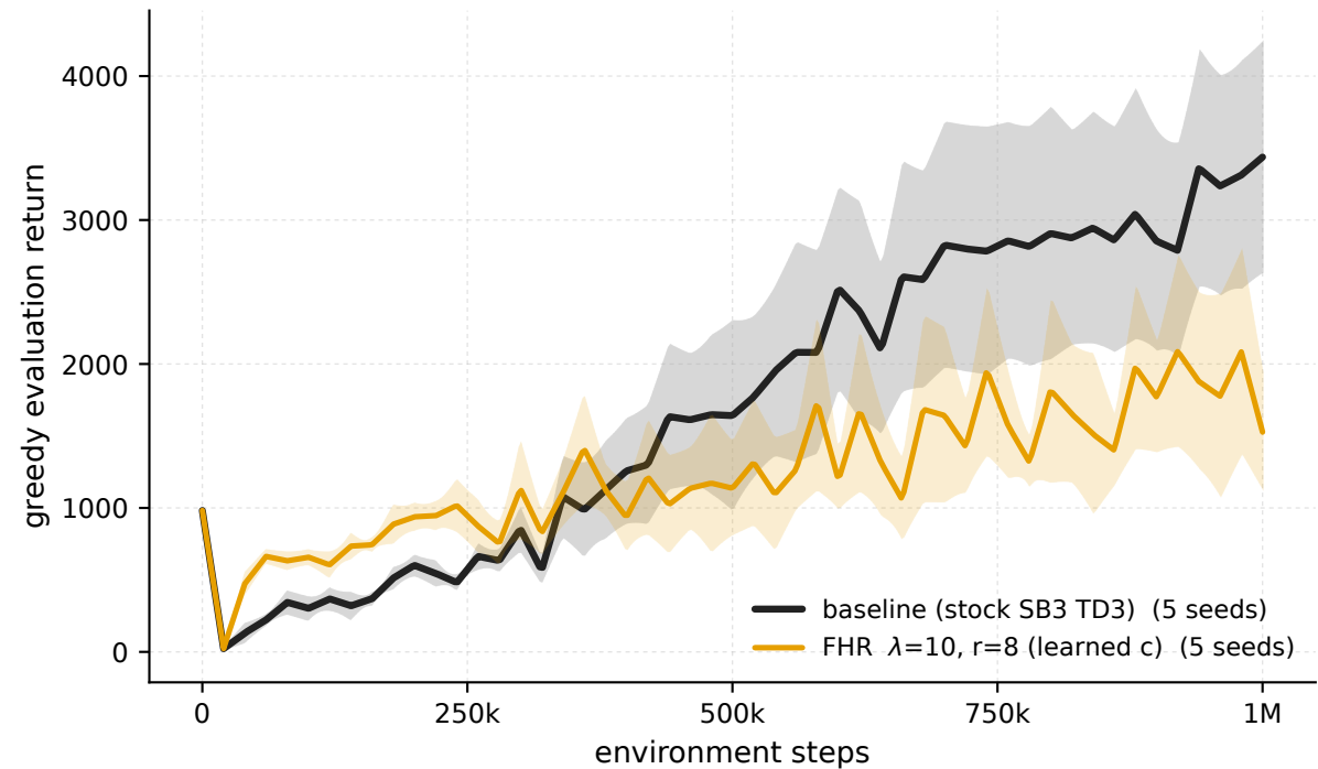
Ant-v5 - \lambda 10 \cdot r8 vs baseline (greedy eval)
