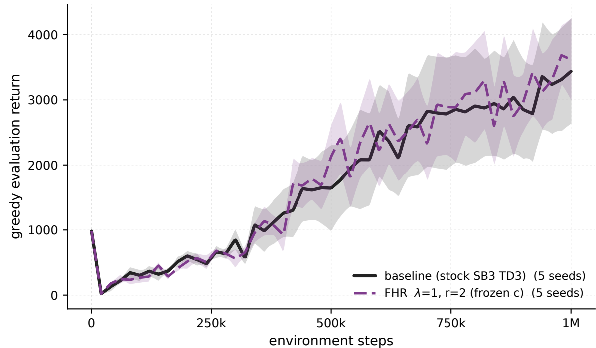
Ant-v5 - \lambda=1, r=2 frozen-c vs baseline (greedy eval)
