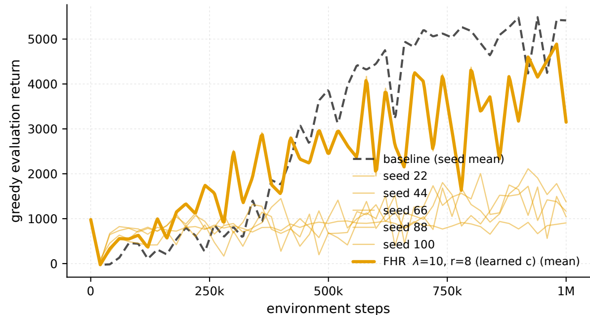
Ant-v5 - \lambda 10 \cdot r8 , every seed (eval)
