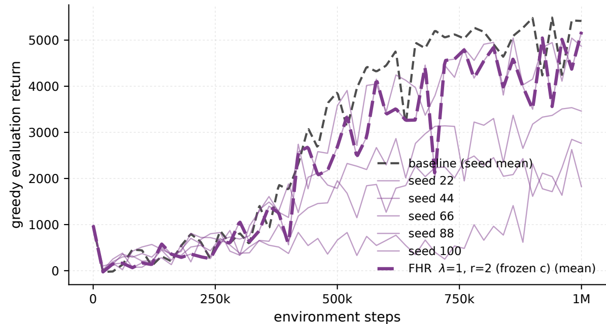
Ant-v5 - \lambda 1 \cdot r 2 frozen-c, every seed (eval)
