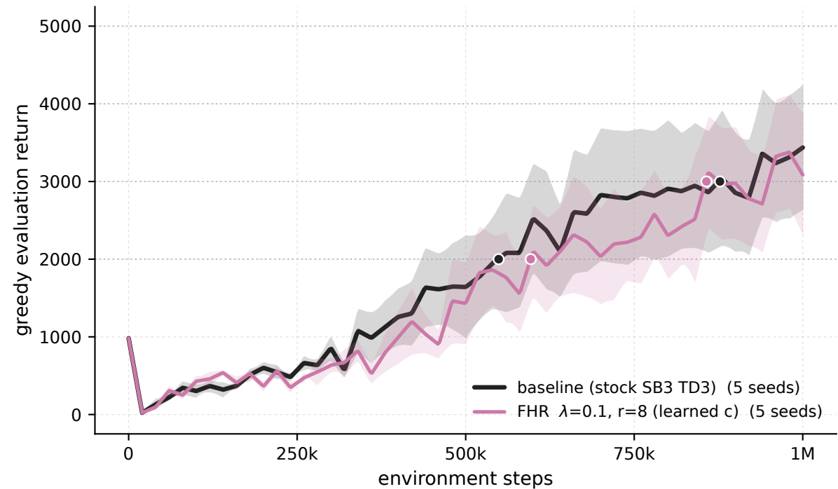
Ant-v5 - \lambda 0.1 \cdot r8 vs baseline (greedy eval)
