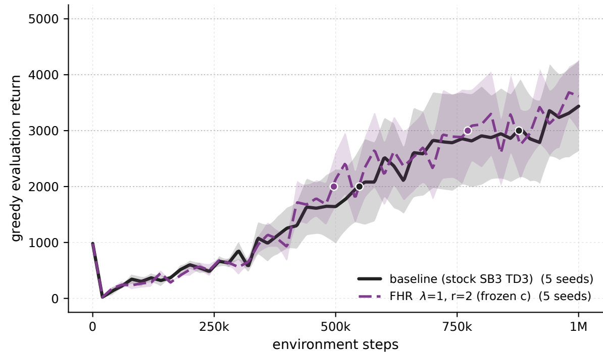
Ant-v5 - \lambda 1 \cdot r2 frozen-c vs baseline (greedy eval)
