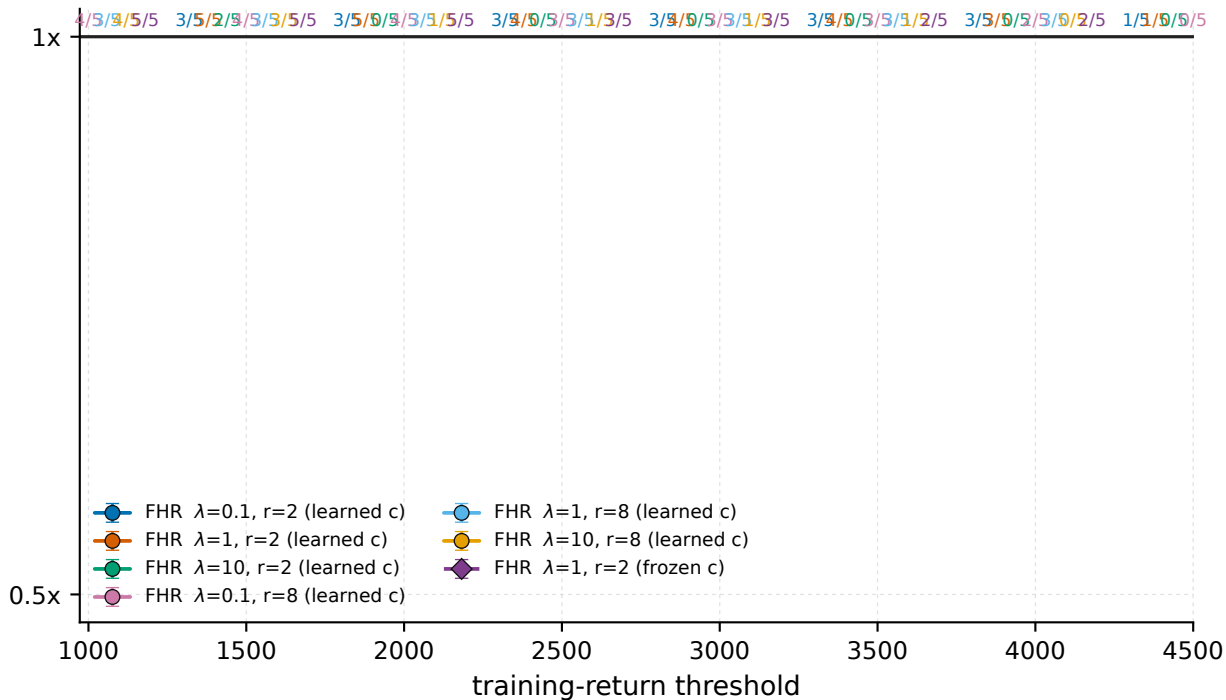
Ant-v5 - paired-bootstrap speed-up (95% CI); 'k/n' = seeds that reached the bar
