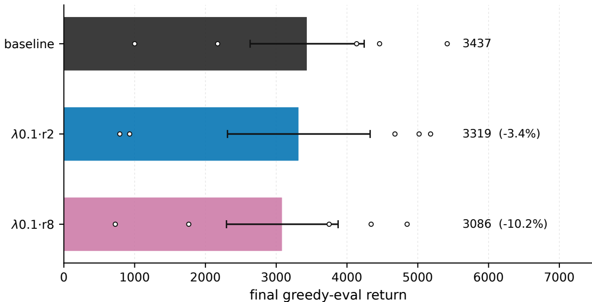
Ant-v5 - final return, \lambda = 0.1 vs baseline
