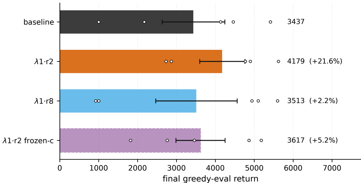
Ant-v5 - final return, \lambda = 1 vs baseline
