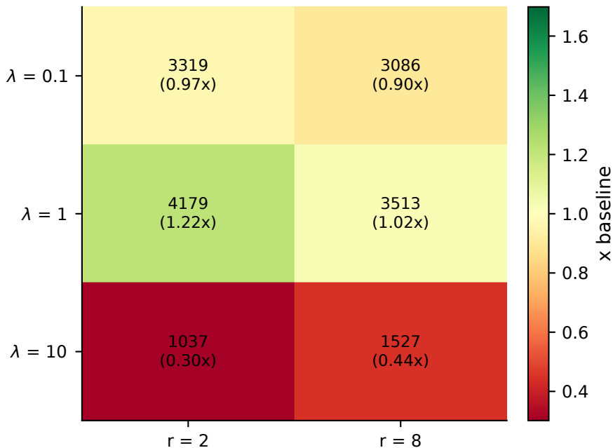
final return vs baseline (3437)
