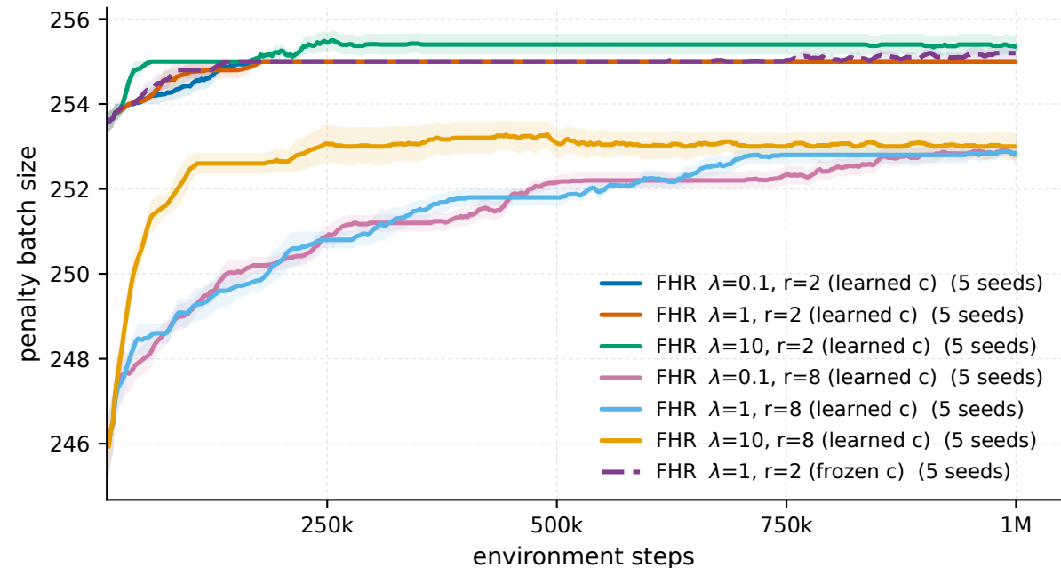
Ant-v5 - penalty batch size
