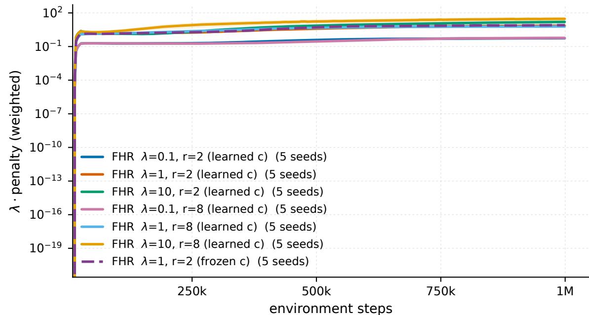
Ant-v5 - \lambda \cdot \text{penalty} (weighted)
