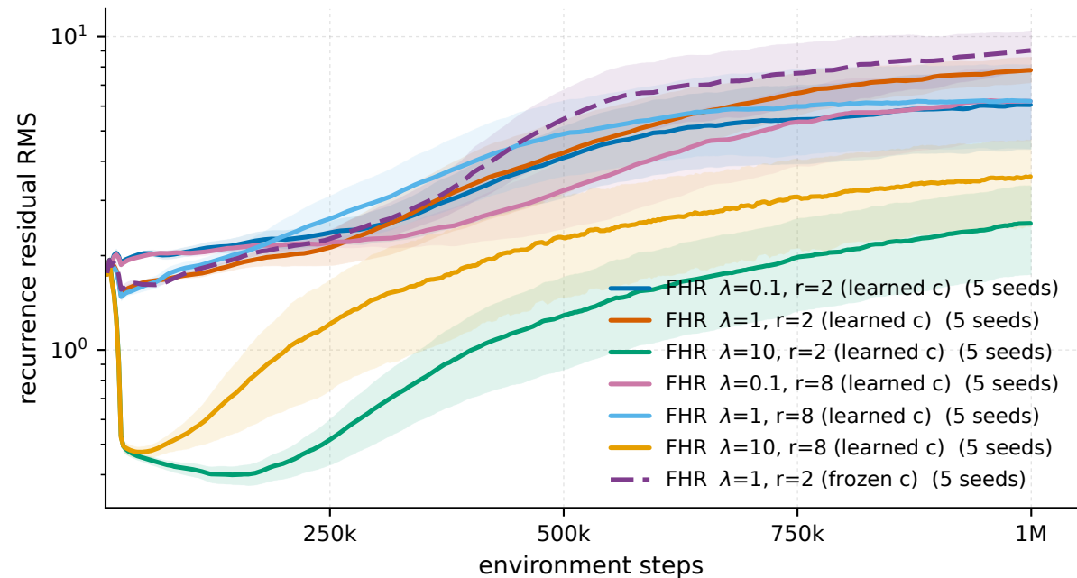
Ant-v5 - recurrence residual RMS
