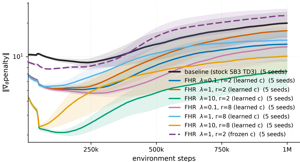
Ant-v5 - \|\nabla_{\theta}\text{penalty}\|
