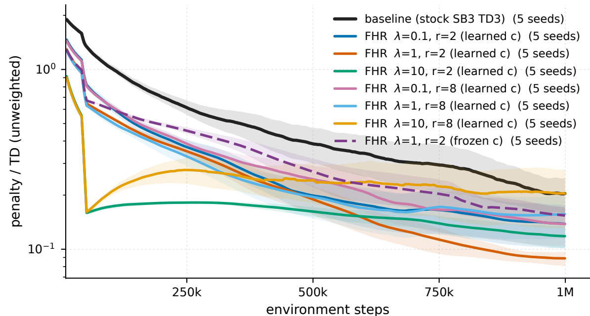
Ant-v5 - penalty / TD (unweighted)
