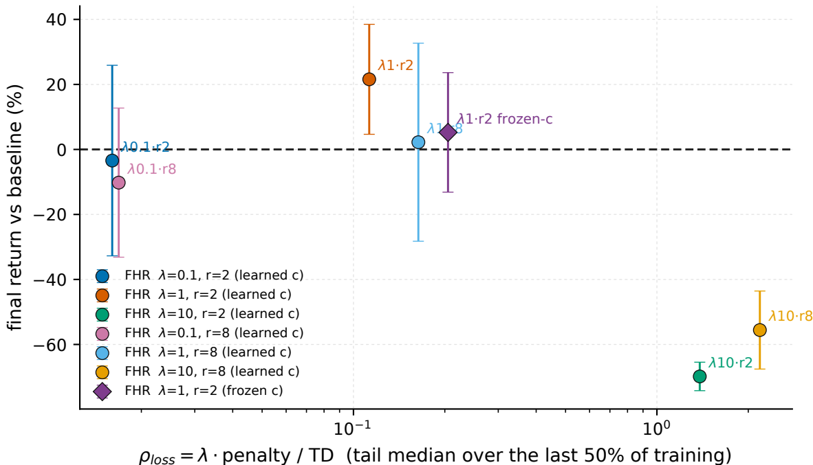
Ant-v5 - how hard the penalty pushes vs what it buys
