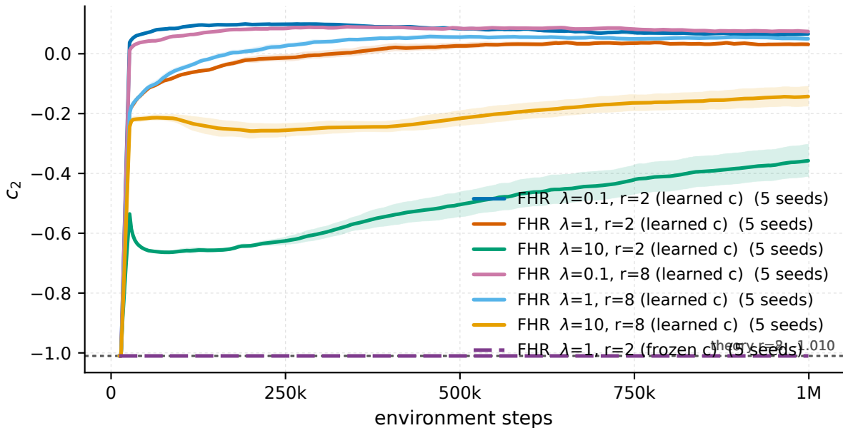
Ant-v5 - recurrence coefficient c_2 vs the Bellman theory value
