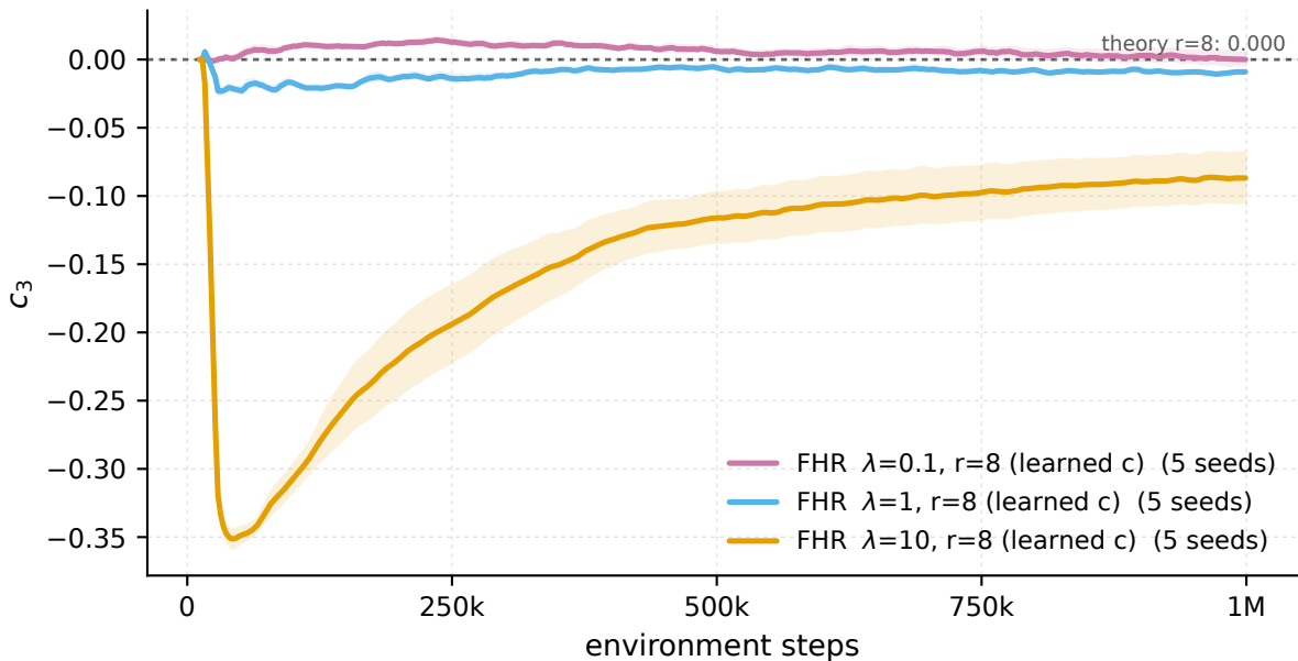
Ant-v5 - recurrence coefficient c_3 vs the Bellman theory value
