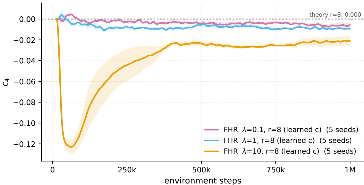
Ant-v5 - recurrence coefficient c_4 vs the Bellman theory value
