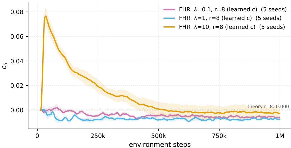
Ant-v5 - recurrence coefficient c_5 vs the Bellman theory value
