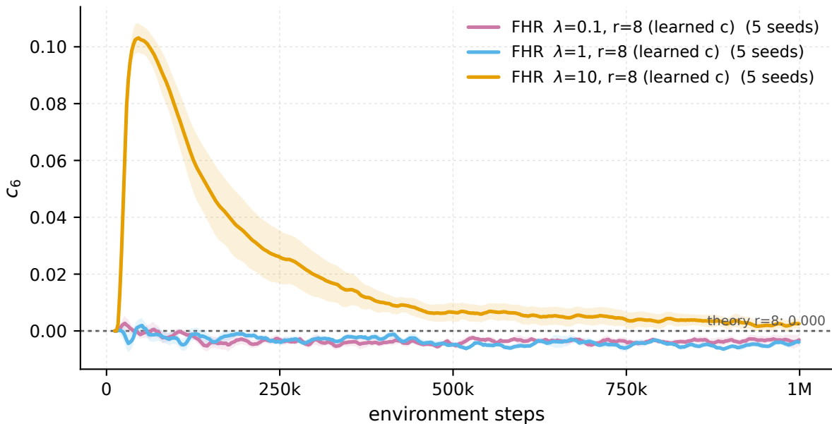
Ant-v5 - recurrence coefficient c_6 vs the Bellman theory value
