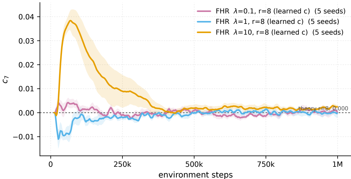
Ant-v5 - recurrence coefficient c_7 vs the Bellman theory value
