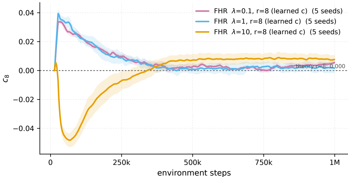
Ant-v5 - recurrence coefficient c_8 vs the Bellman theory value
