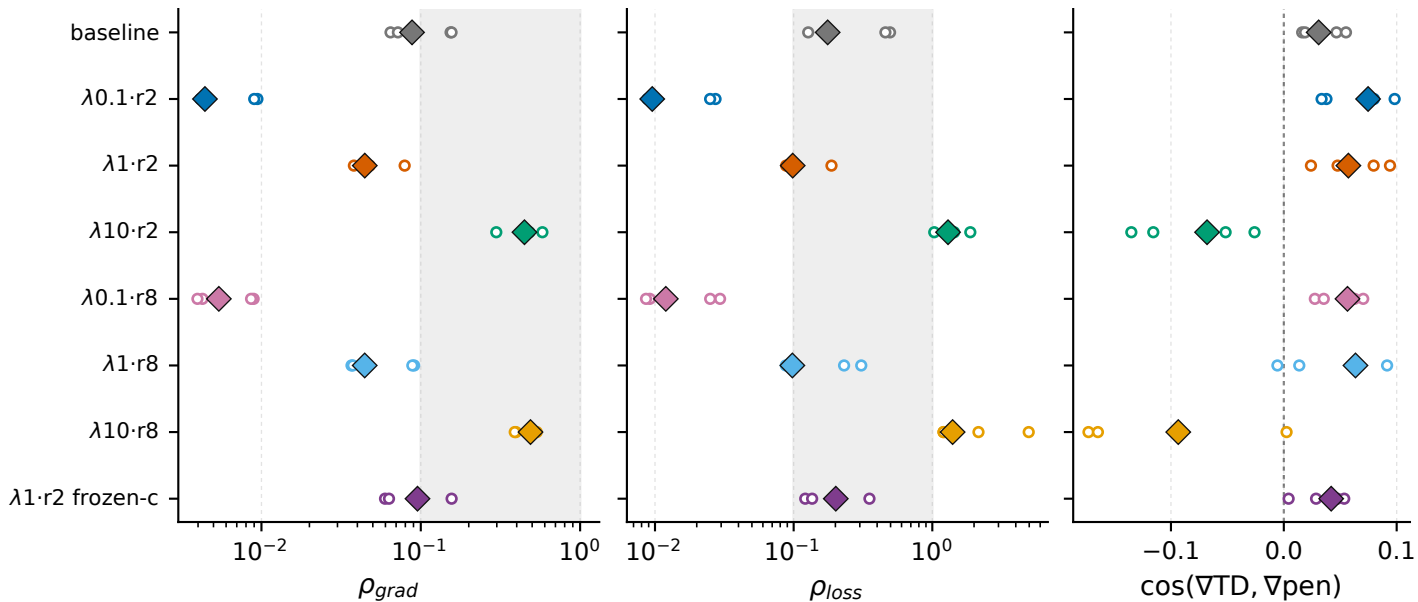
Ant-v5 - stream ratios, tail medians over the last 50% (baseline: unweighted); shaded = target range
