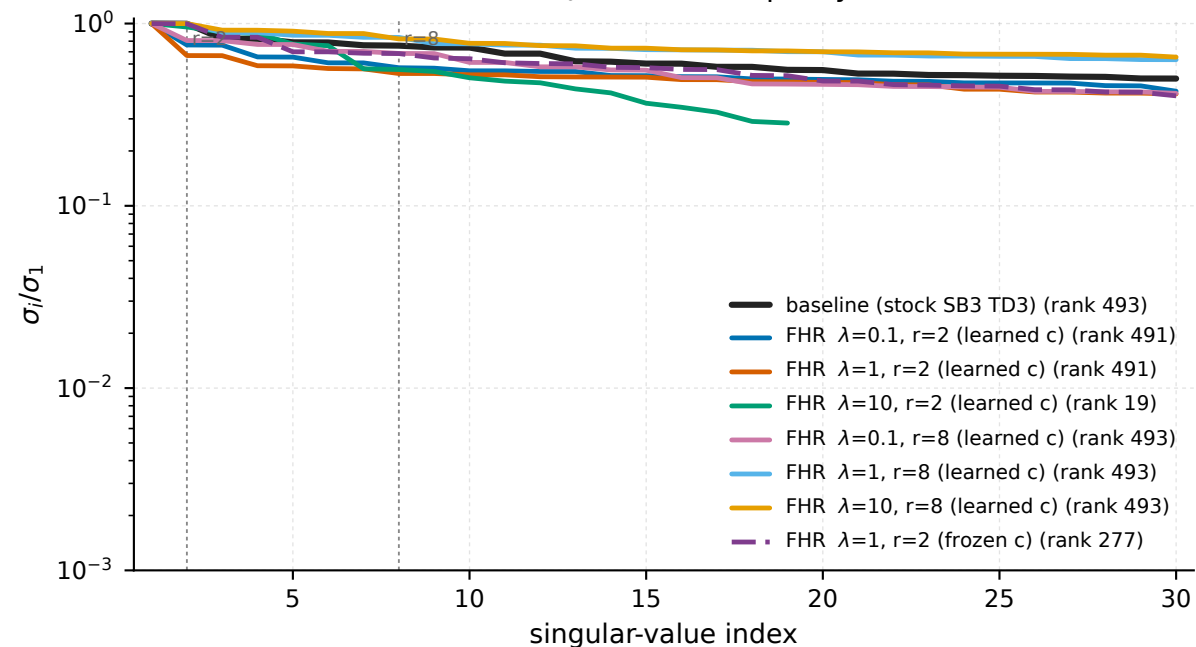
Ant-v5 - Hankel( \pi(s_t)_0 ) of the final policy (action dim 0)
