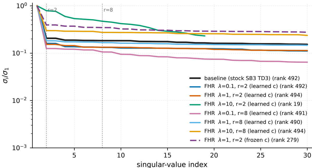
Ant-v5 - Hankel( \pi(s_t)_1 ) of the final policy (action dim 1)
