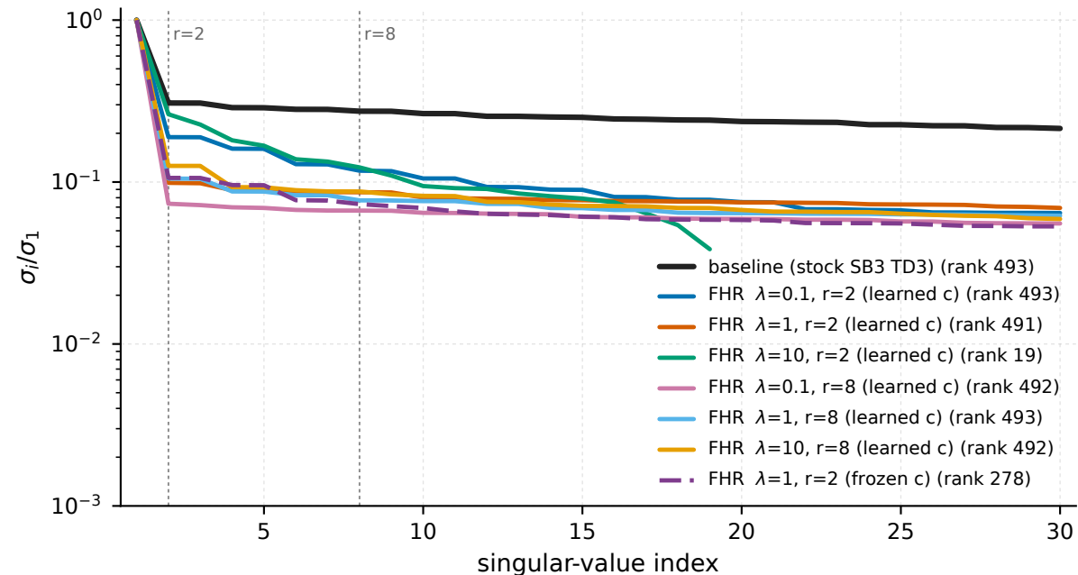
Ant-v5 - \text{Hankel}(\pi(s_t)_2) of the final policy (action dim 2)
