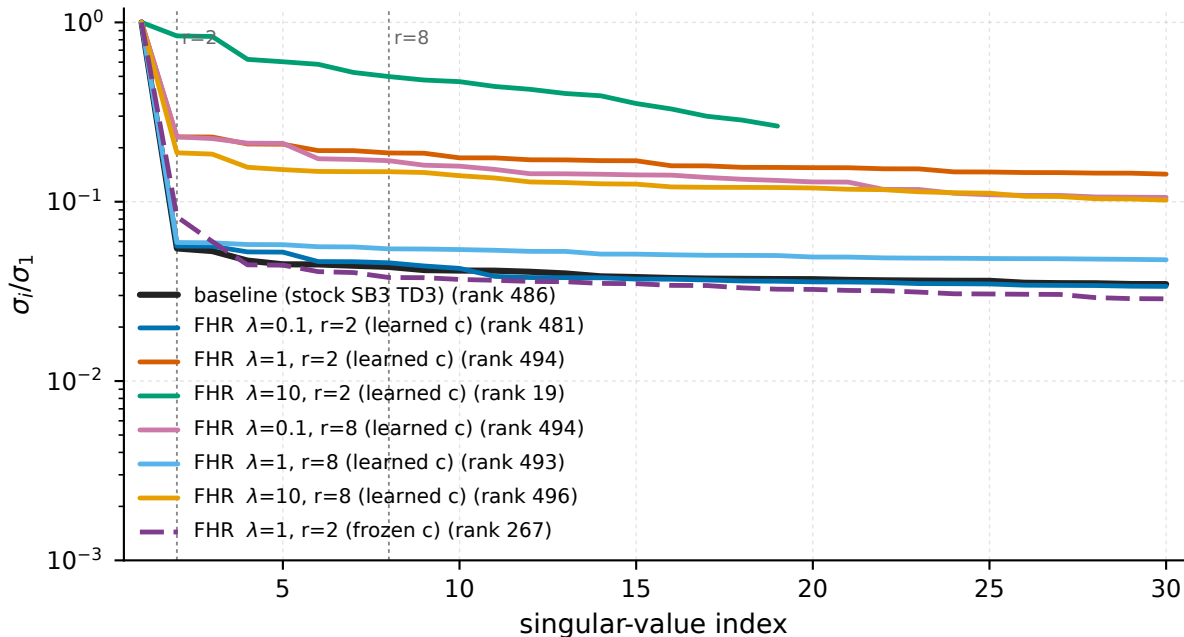
Ant-v5 - Hankel( \pi(s_t)_6 ) of the final policy (action dim 6)
