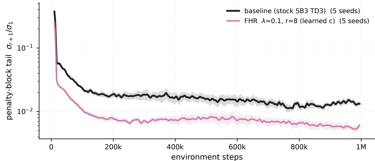
Ant-v5 - \lambda 0.1 \cdot r8 vs baseline, penalised windows penalty-block tail \sigma_{r+1}/\sigma_1
