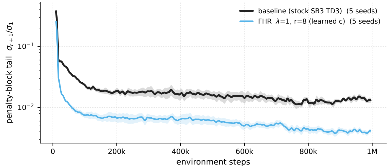
Ant-v5 - \lambda 1 \cdot r 8 vs baseline, penalised windows penalty-block tail \sigma_{r+1}/\sigma_1
